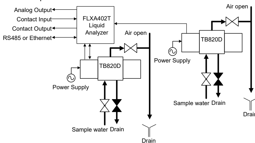
FLXA402T 2nd input “-P1” or “-C1”
